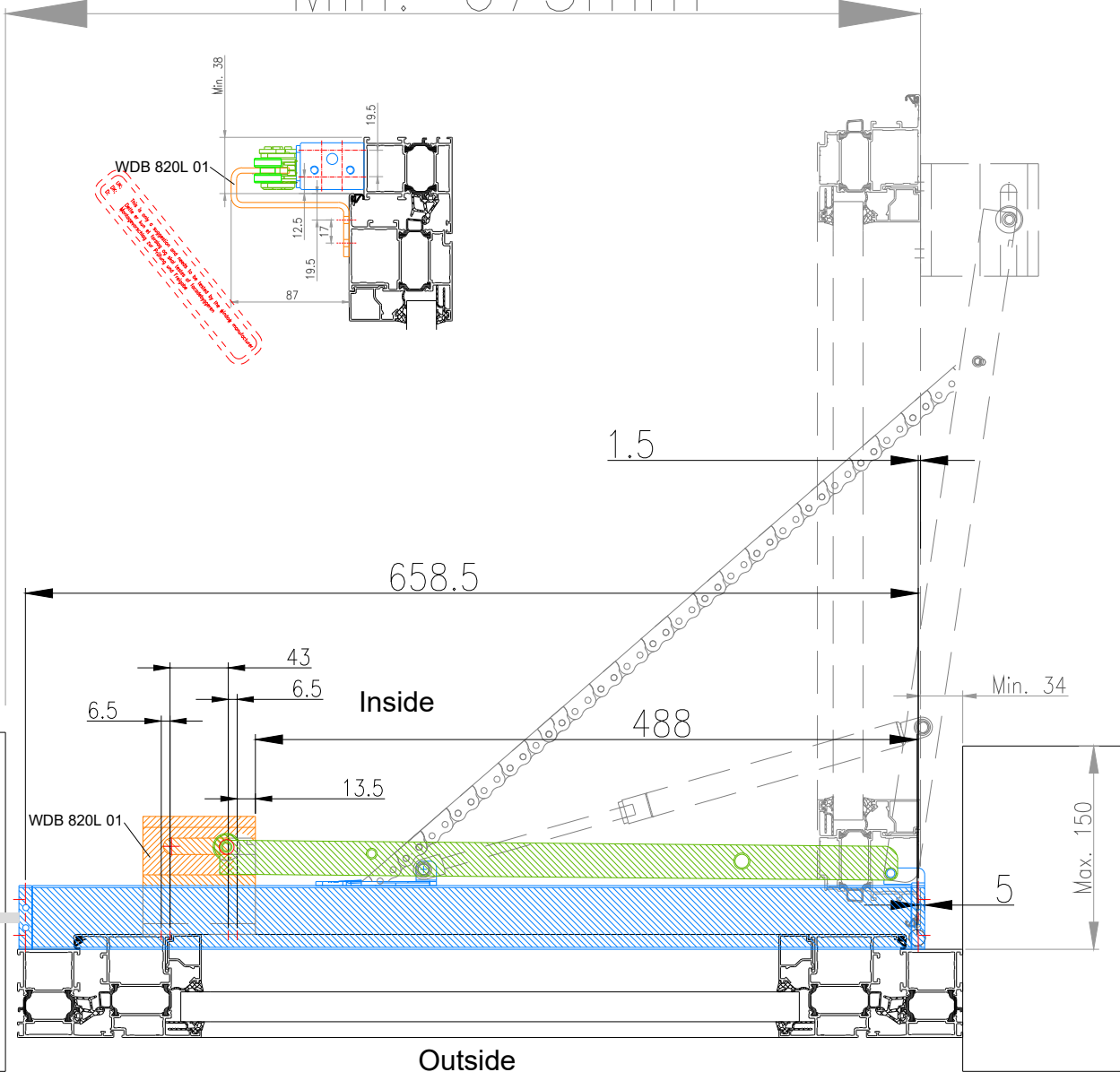
WDB 820L 01 in Principle sketch
