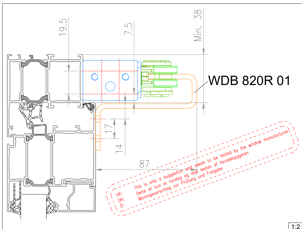
WDB 820R 01 in Principle sketch
