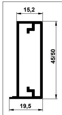
Glassmass = Rahmen -4 mm
